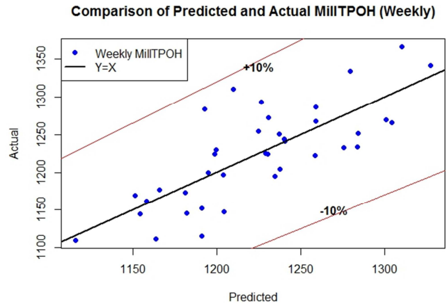
Figure 6. 10% error range.
